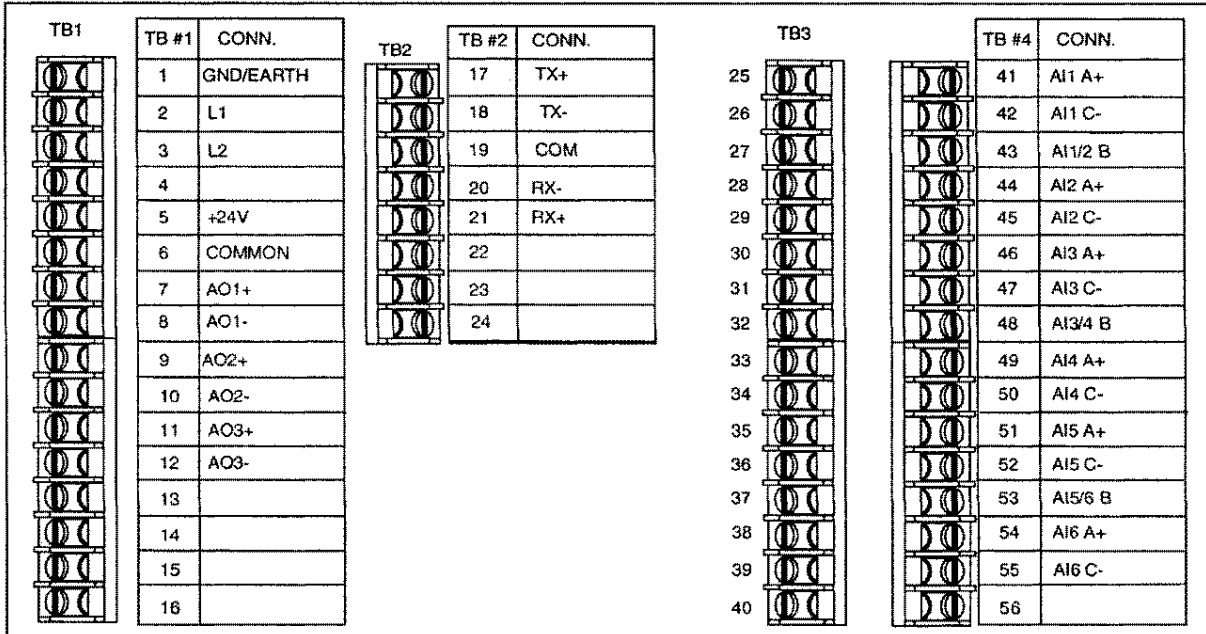
Figure 0-1 Terminal Connections
