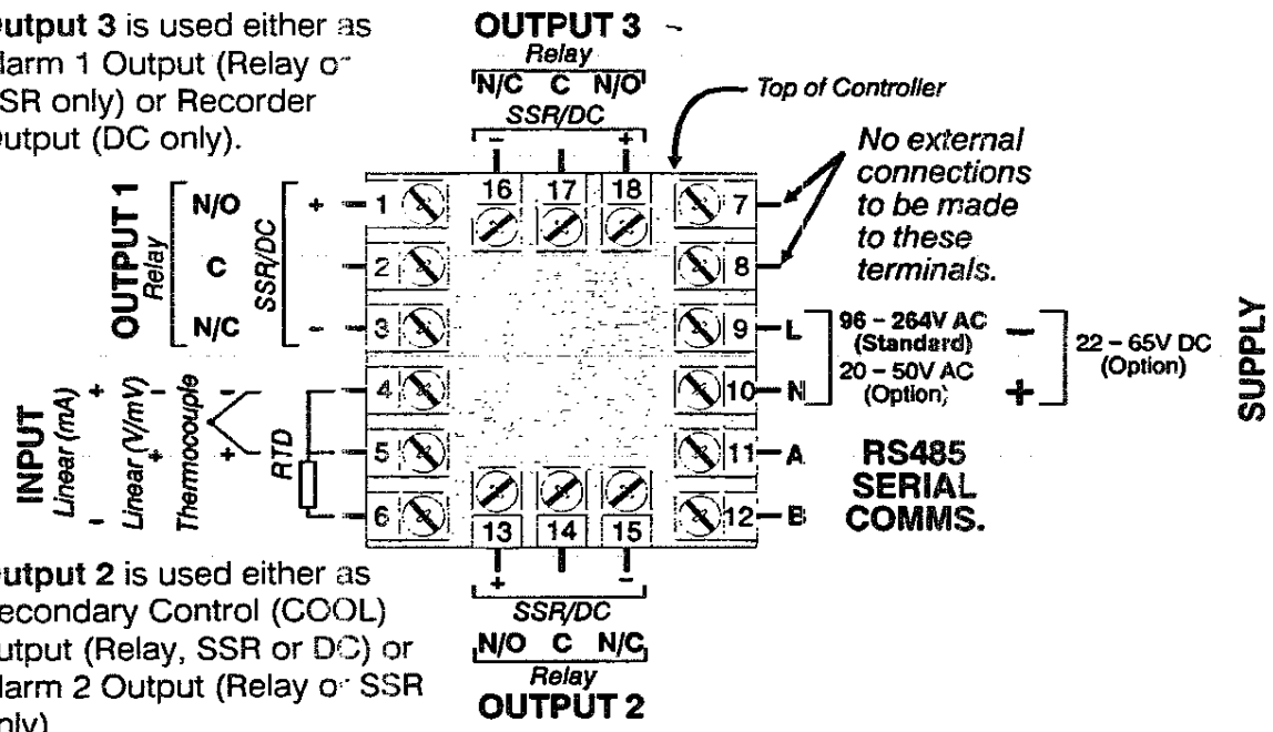
Figure 3-4 Rear Terminal Connections
