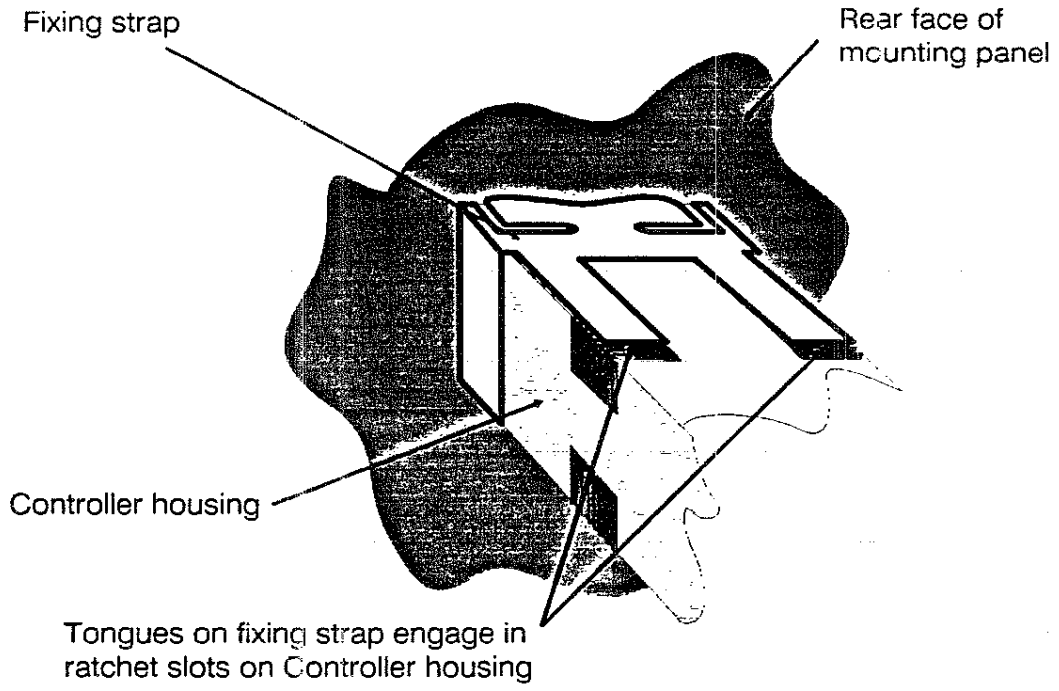
Figure 3-3 Panel-mounting the Controller
