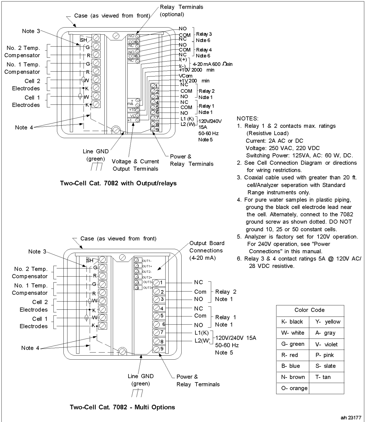
Figure 0-1 Terminal Connections
