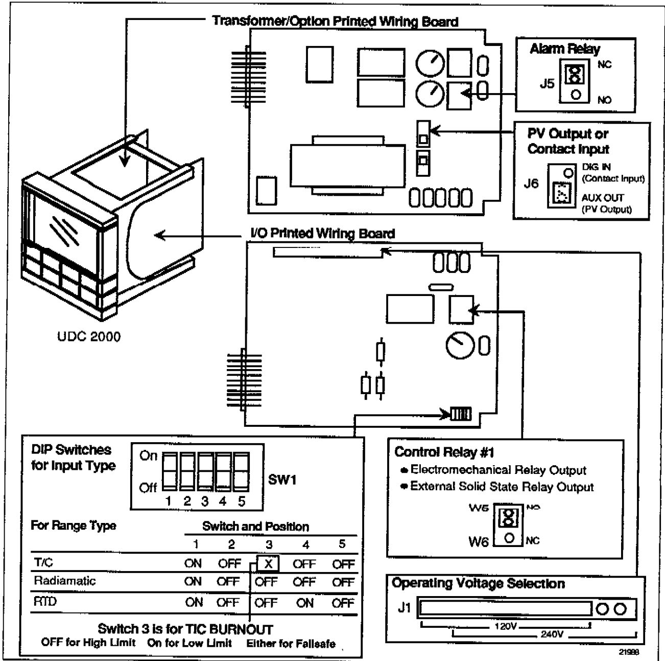
Figure 2-2 Jumper Placement and Switch Settings
