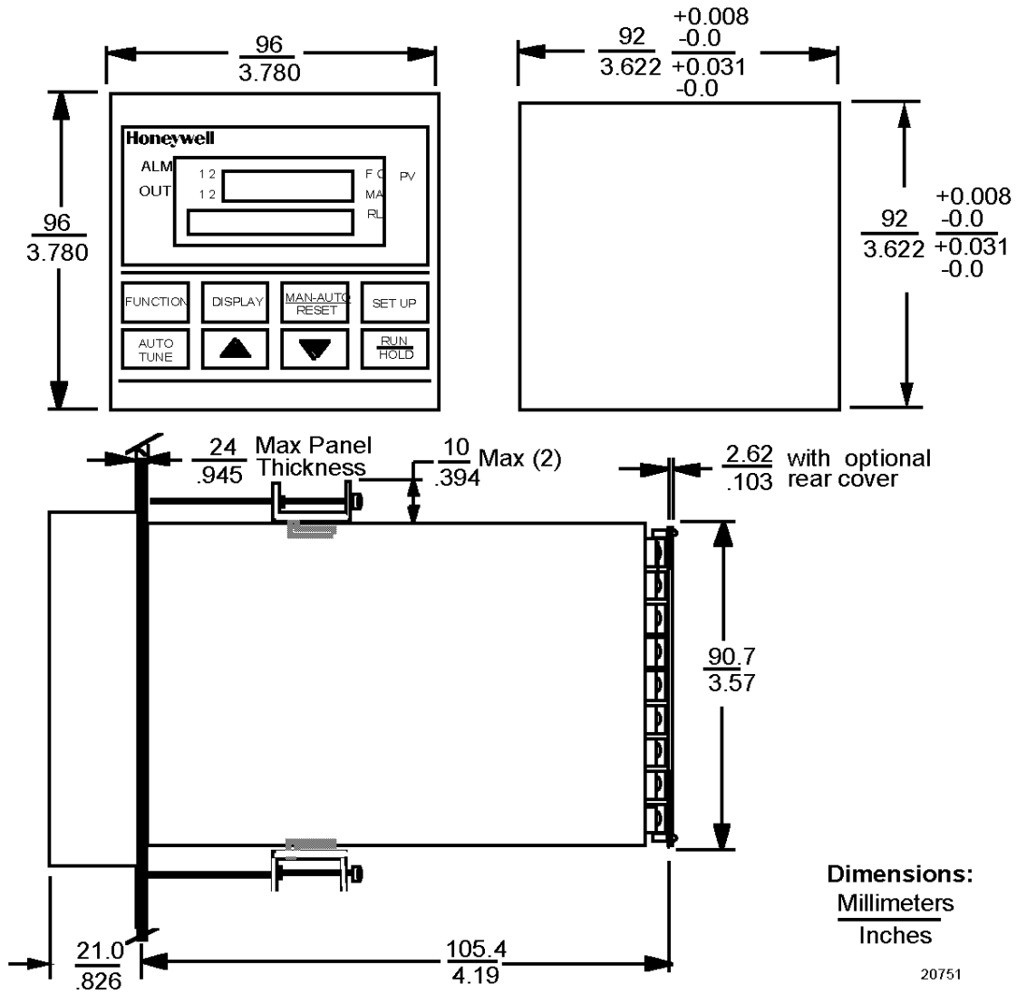
Figure 5—UDC 2300 Controller Dimensions – not to scale
